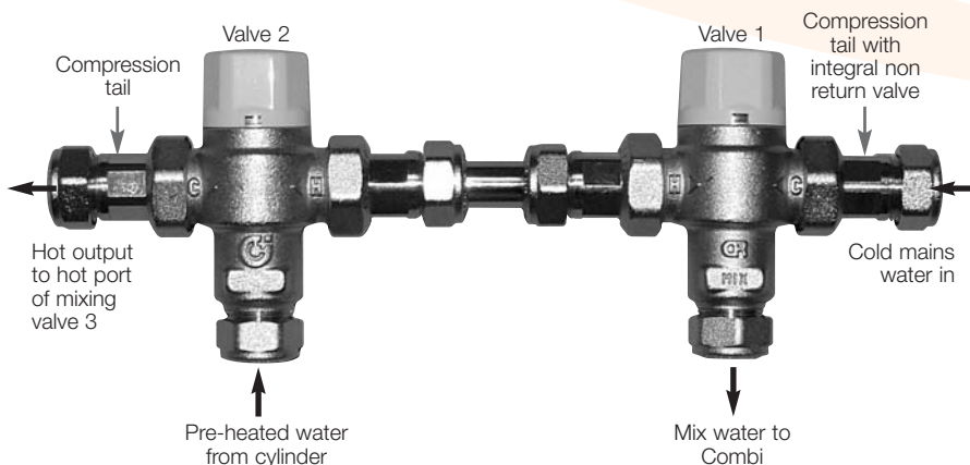
Figure 1: Temperature control manifold
